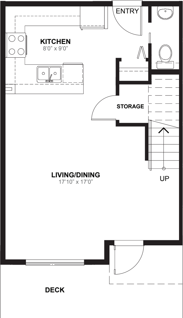
2ND FLOOR PLAN (MAIN FLOOR)
