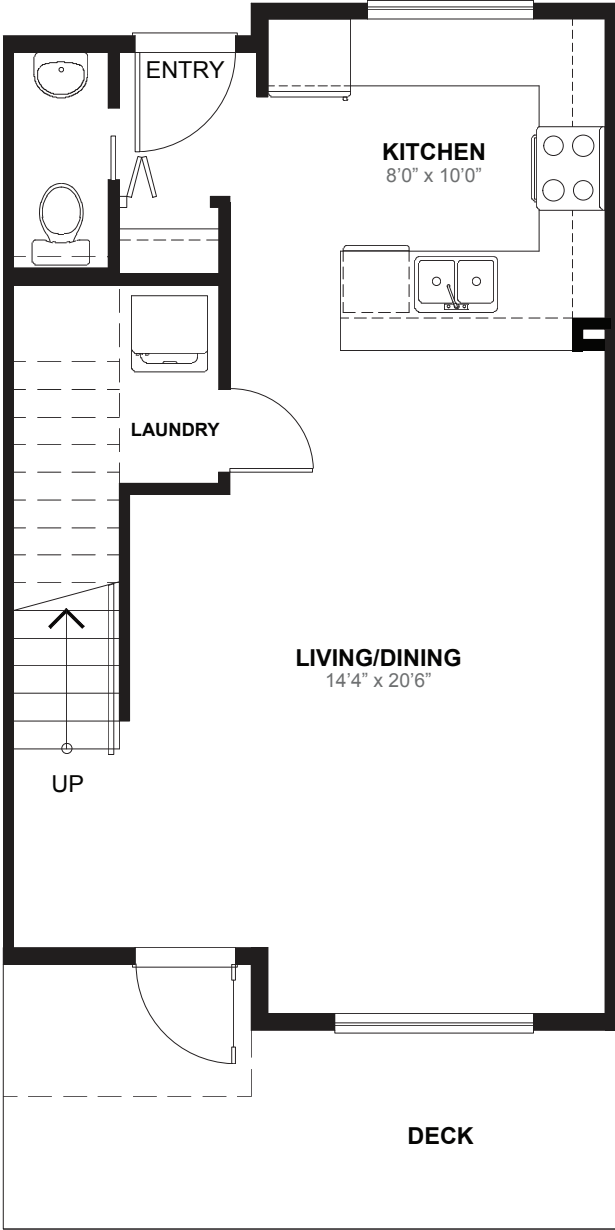
2ND FLOOR PLAN (MAIN FLOOR)
